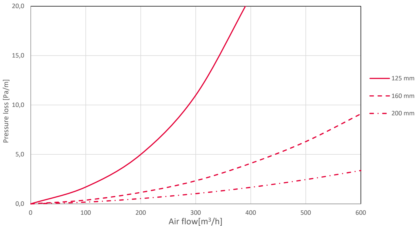
Pressure loss - Duct silencer ARIA ADURO
